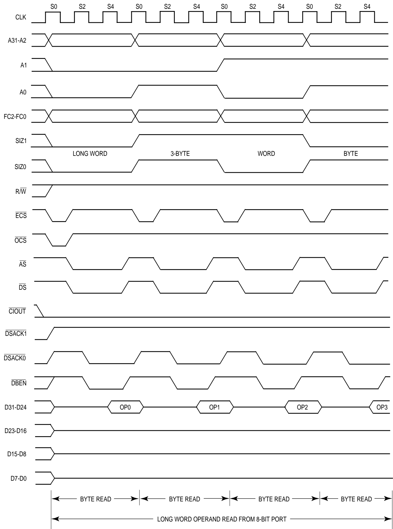
Figure 7-22. Long-Word Read — 8-Bit Port with \overline{\text{CIOUT}} Asserted
